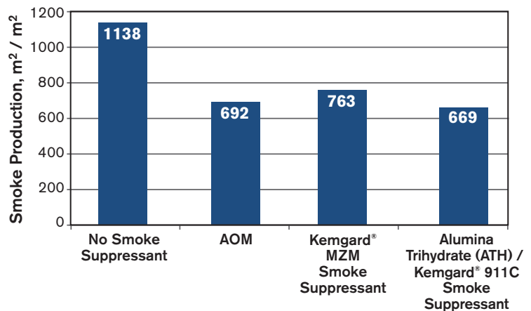
ISO 5660 Total Smoke in Rigid PVC Compound
